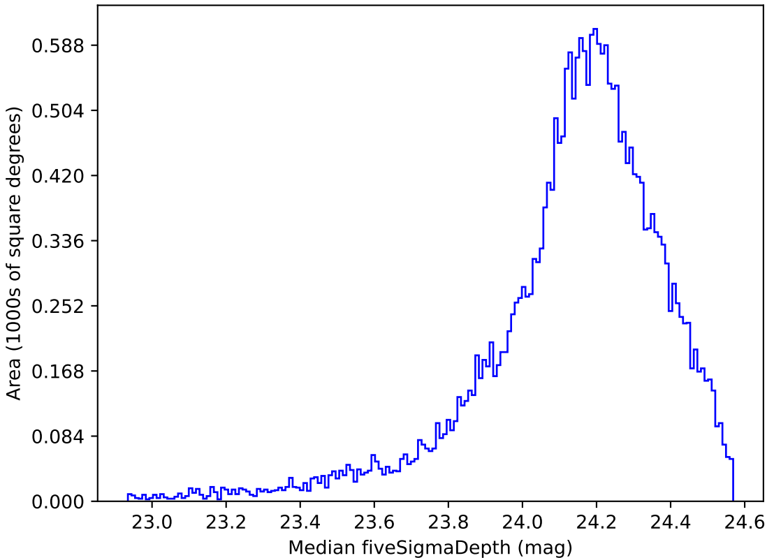
weather_cloudso31v3.4_10yrs Yr 1 r band: Median fiveSigmaDepth
