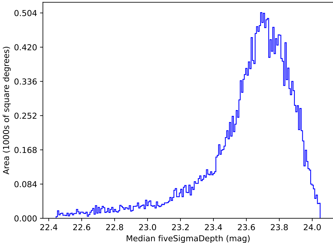
weather_cloudso31v3.4_10yrs Yr 1 i band: Median fiveSigmaDepth
