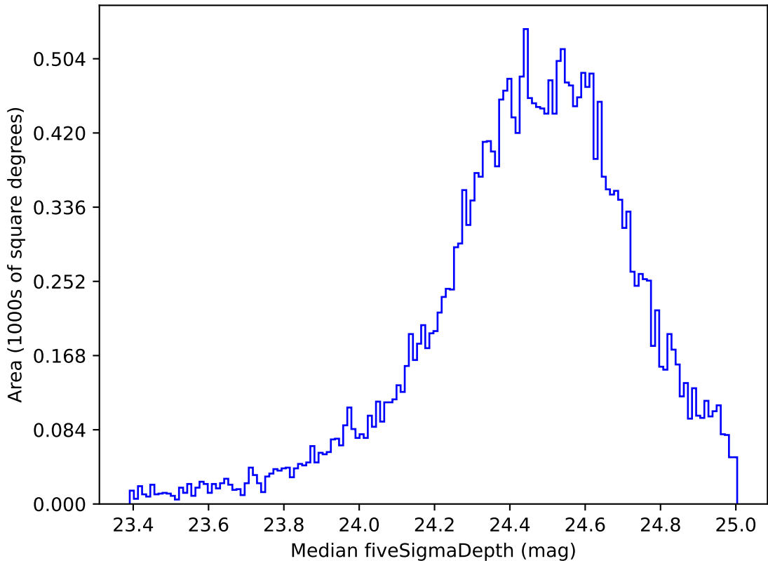
weather_cloudso31v3.4_10yrs Yr 1 g band: Median fiveSigmaDepth
