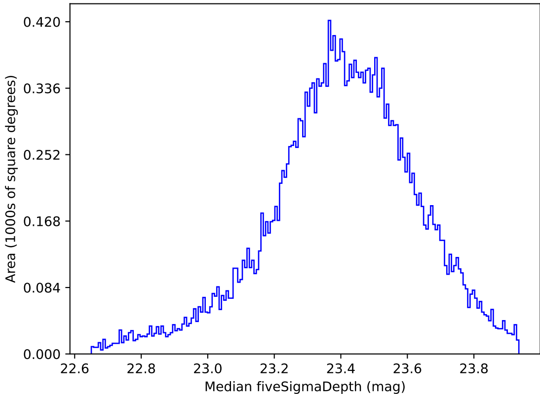
weather_cloudso31v3.4_10yrs Yr 1 all bands: Median fiveSigmaDepth
