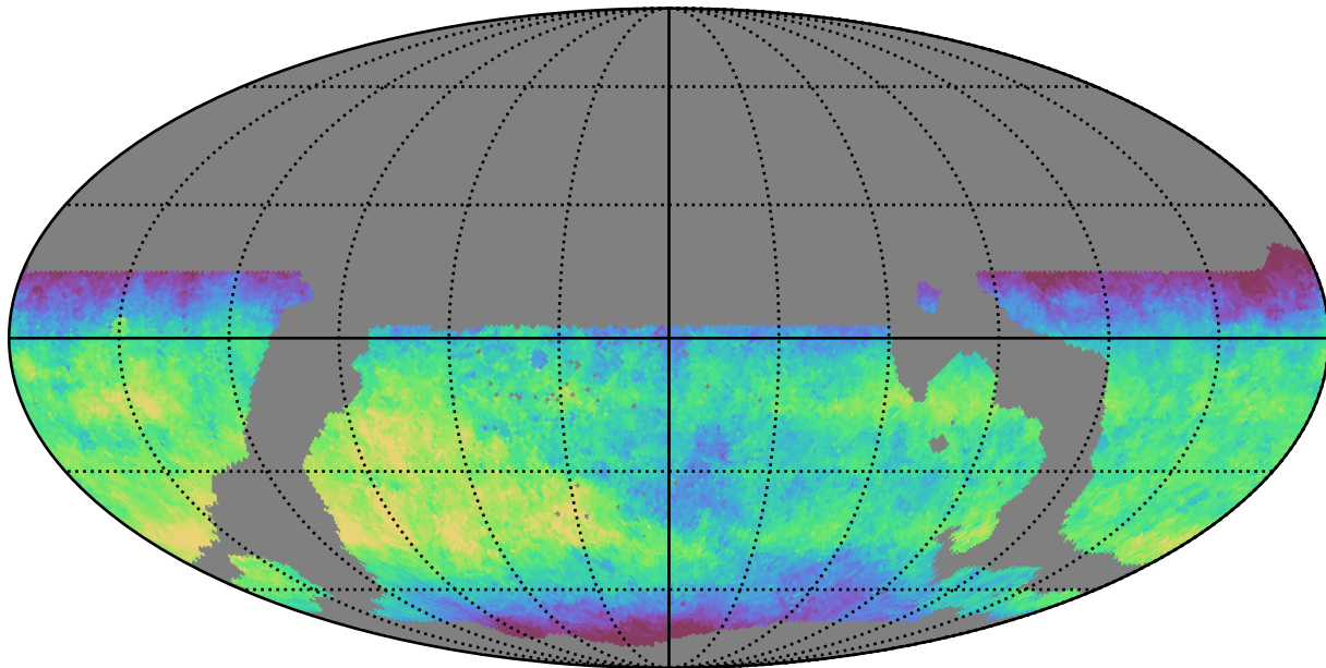
weather_cloudso31v3.4_10yrs WFD z band: Median fiveSigmaDepth
