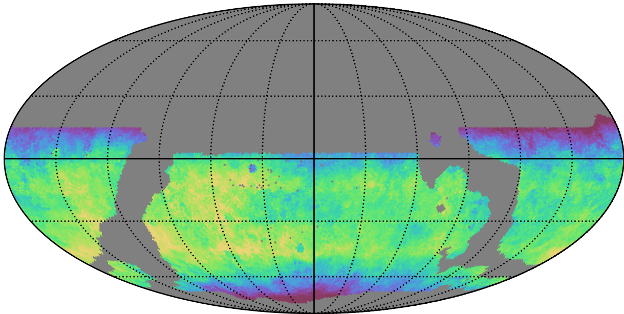
weather_cloudso31v3.4_10yrs WFD y band: Median fiveSigmaDepth
