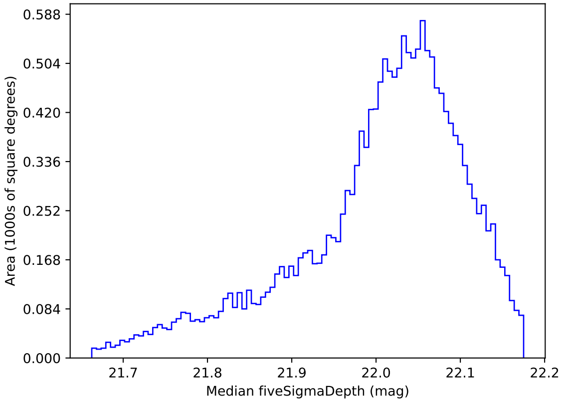
weather_cloudso31v3.4_10yrs WFD y band: Median fiveSigmaDepth
