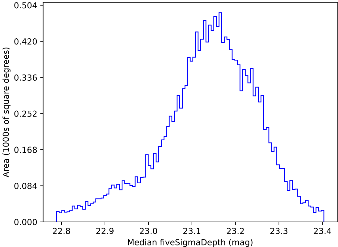
weather_cloudso31v3.4_10yrs WFD u band: Median fiveSigmaDepth
