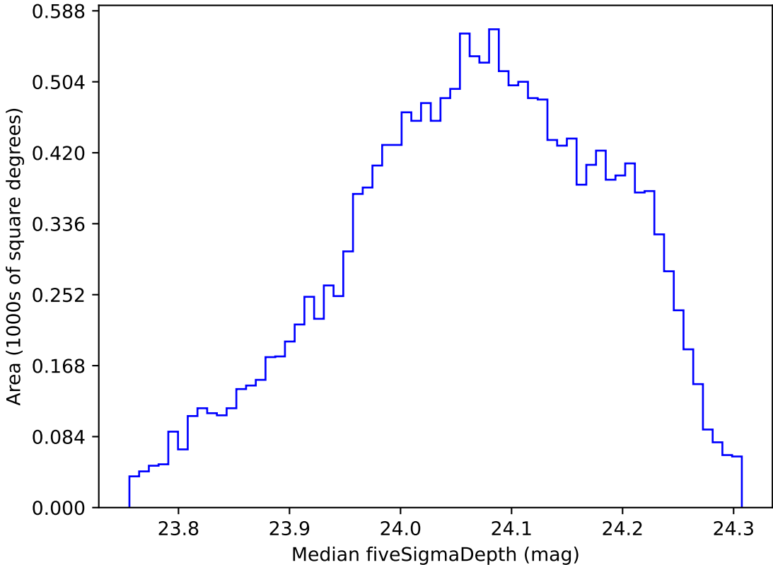
weather_cloudso31v3.4_10yrs WFD r band: Median fiveSigmaDepth
