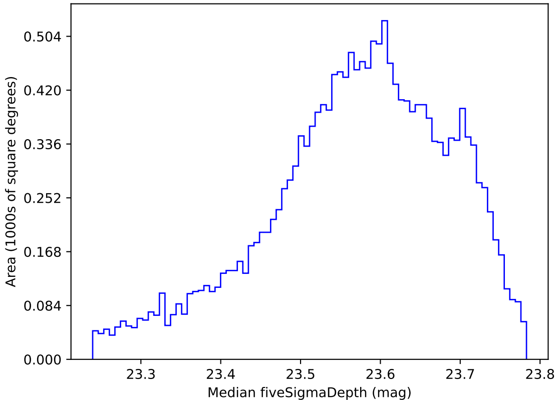
weather_cloudso31v3.4_10yrs WFD i band: Median fiveSigmaDepth
