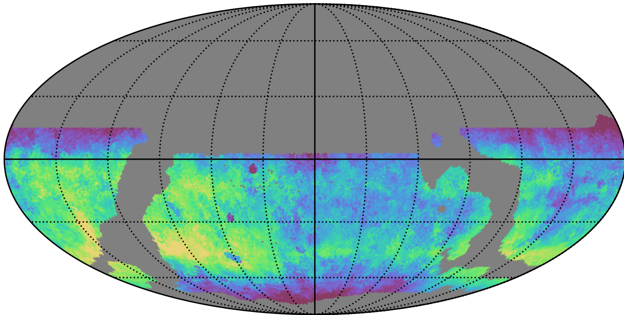
weather_cloudso31v3.4_10yrs WFD g band: Median fiveSigmaDepth
