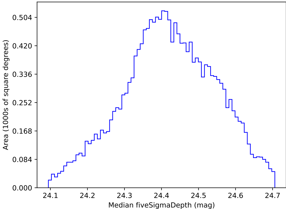
weather_cloudso31v3.4_10yrs WFD g band: Median fiveSigmaDepth
