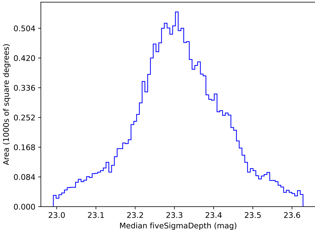
weather_cloudso31v3.4_10yrs WFD all bands: Median fiveSigmaDepth
