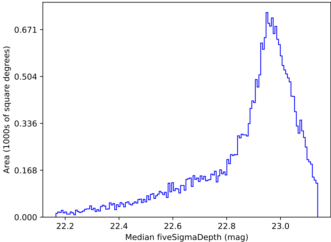
weather_cloudso31v3.4_10yrs All sky z band: Median fiveSigmaDepth
