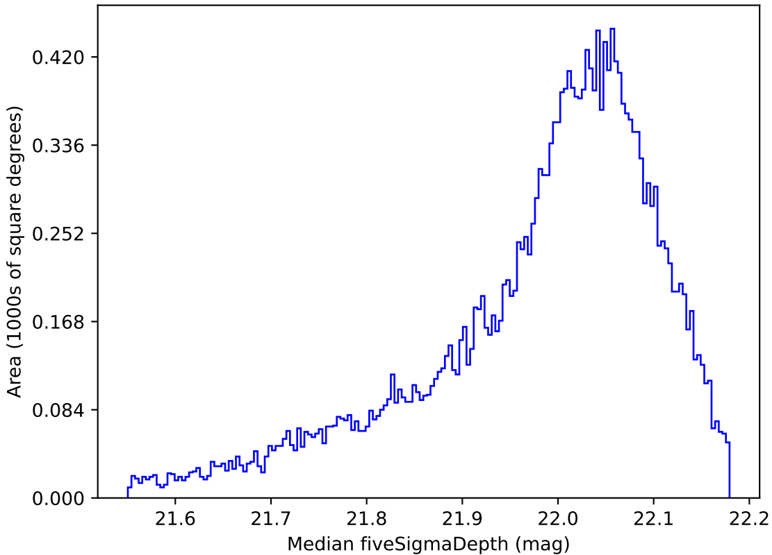
weather_cloudso31v3.4_10yrs All sky y band: Median fiveSigmaDepth
