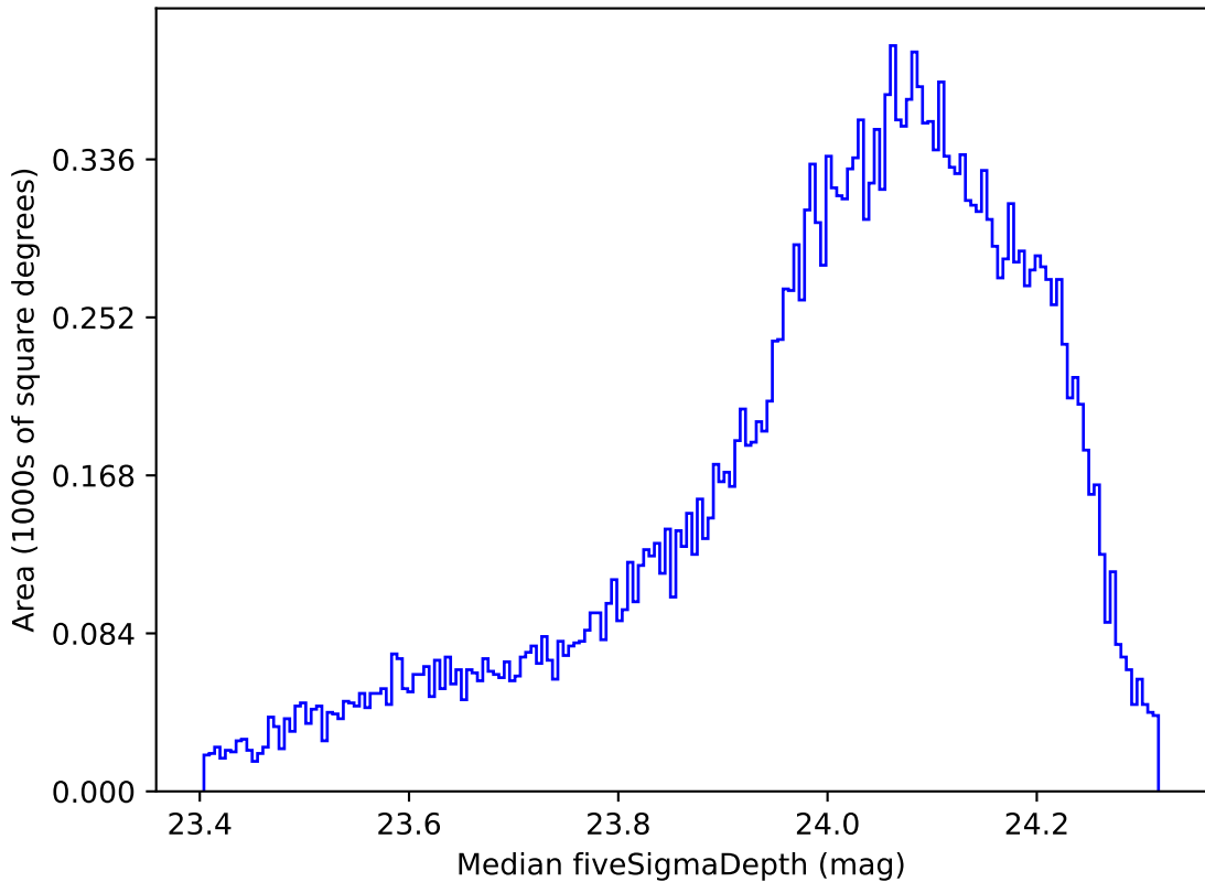
weather_cloudso31v3.4_10yrs All sky r band: Median fiveSigmaDepth
