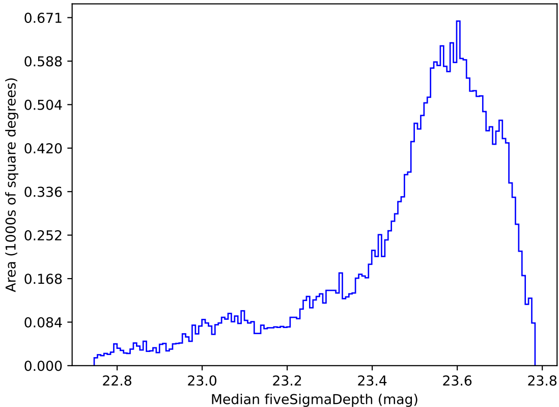
weather_cloudso31v3.4_10yrs All sky i band: Median fiveSigmaDepth
