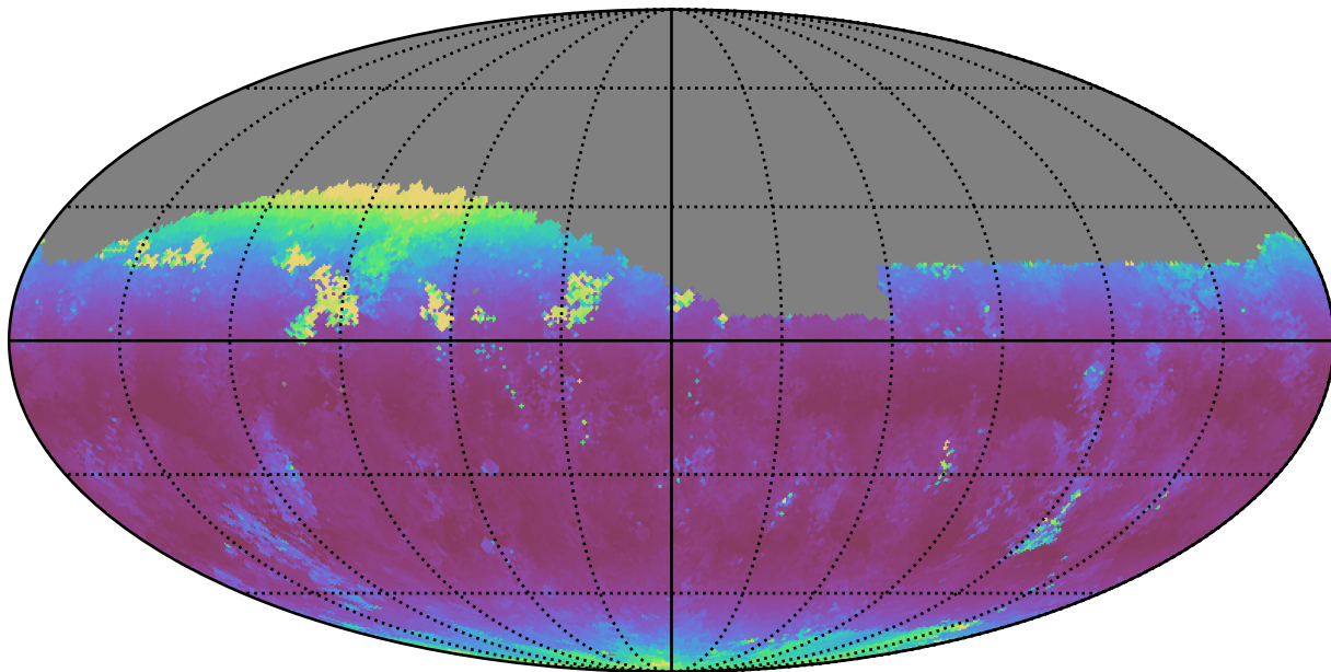
weather_cloudso31v3.4_10yrs Yr 1 z band: Median airmass
