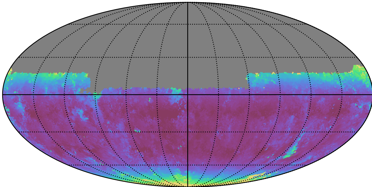
weather_cloudso31v3.4_10yrs Yr 1 y band: Median airmass
