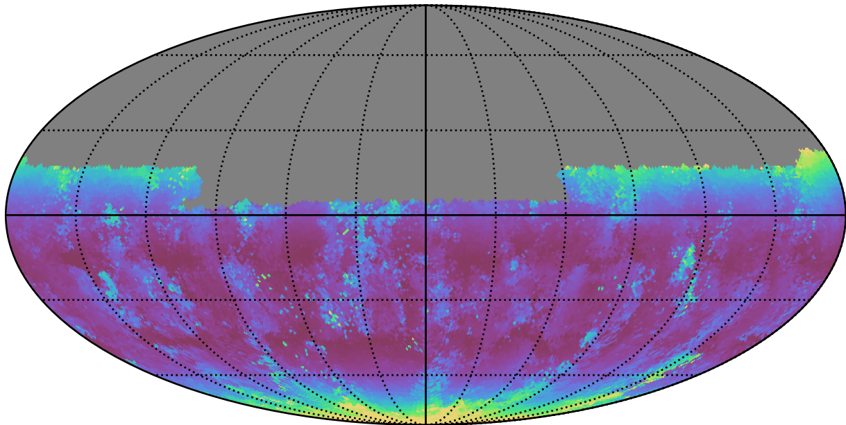
weather_cloudso31v3.4_10yrs Yr 1 u band: Median airmass
