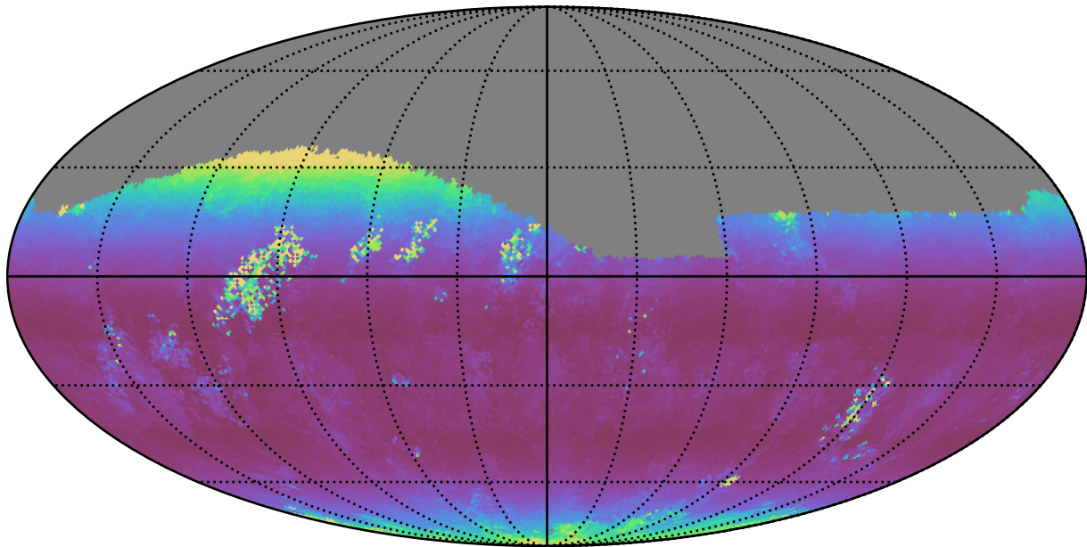
weather_cloudso31v3.4_10yrs Yr 1 r band: Median airmass
