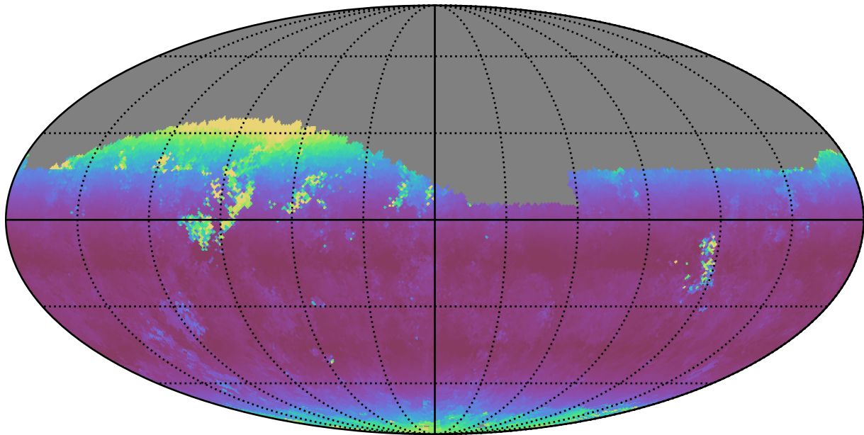
weather_cloudso31v3.4_10yrs Yr 1 i band: Median airmass
