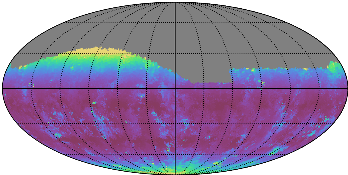
weather_cloudso31v3.4_10yrs Yr 1 g band: Median airmass
