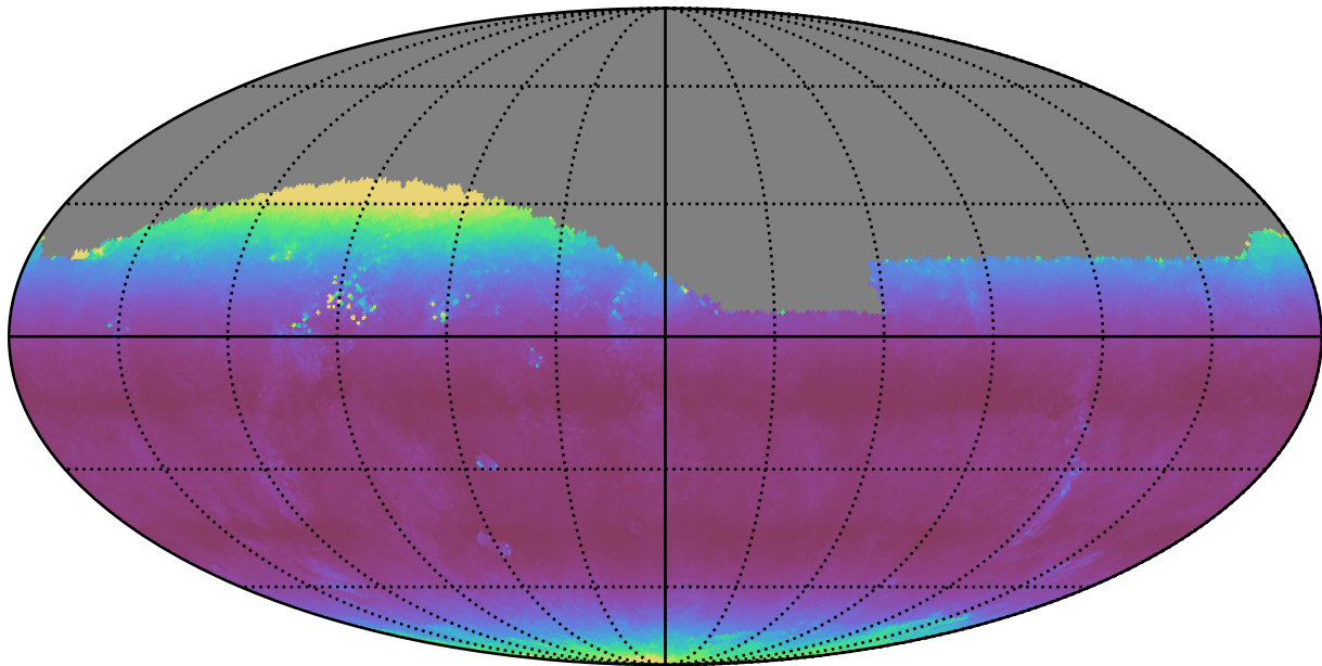
weather_cloudso31v3.4_10yrs Yr 1 all bands: Median airmass
