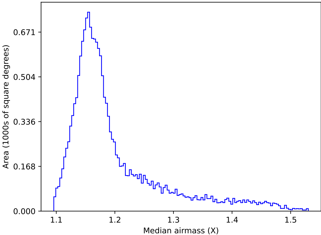
weather_cloudso31v3.4_10yrs WFD z band: Median airmass
