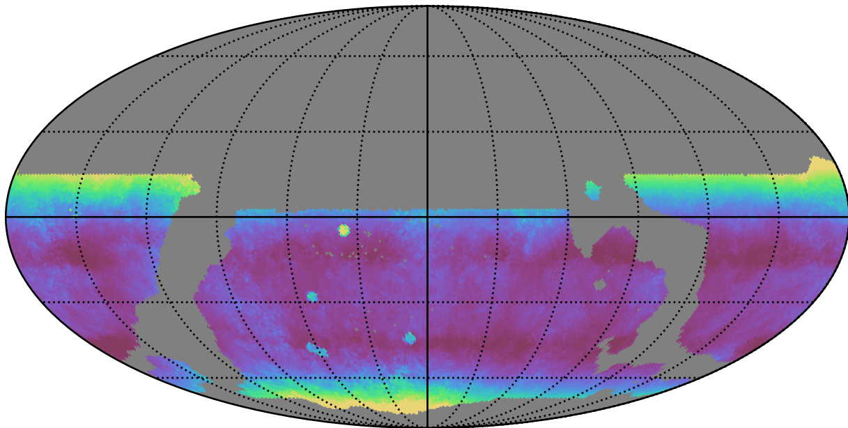
weather_cloudso31v3.4_10yrs WFD y band: Median airmass
