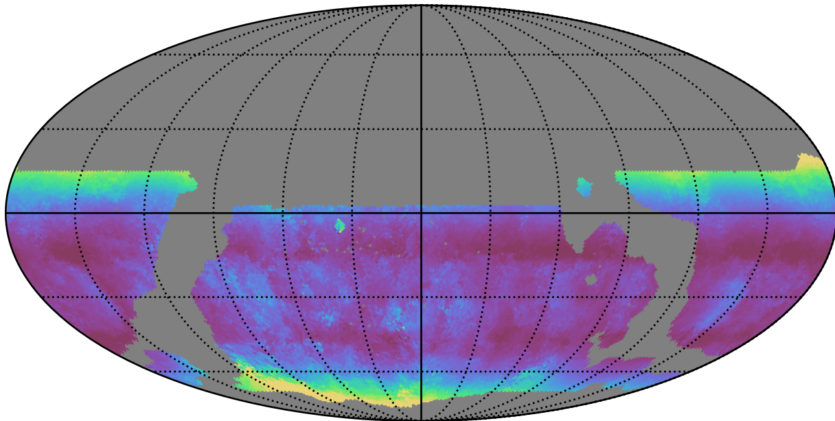
weather_cloudso31v3.4_10yrs WFD u band: Median airmass
