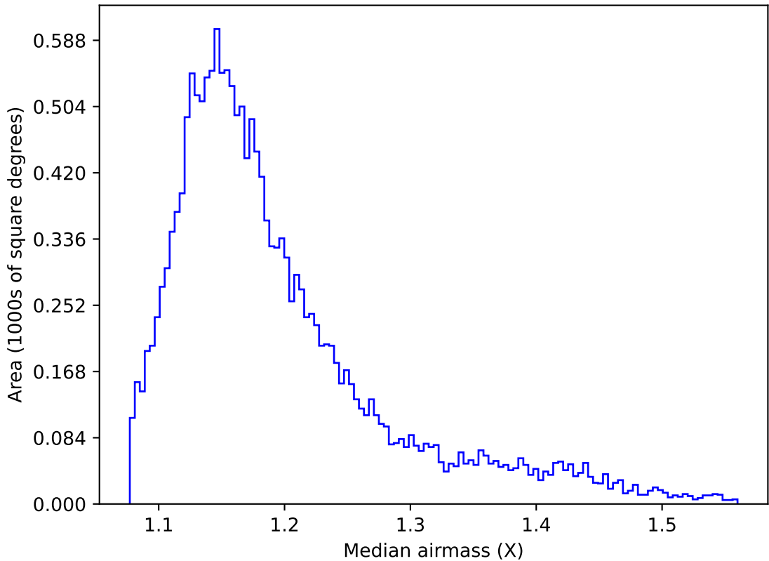
weather_cloudso31v3.4_10yrs WFD u band: Median airmass
