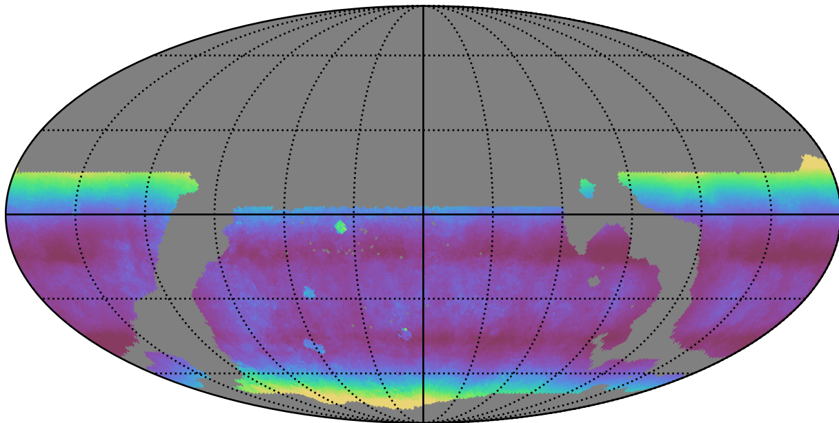
weather_cloudso31v3.4_10yrs WFD r band: Median airmass
