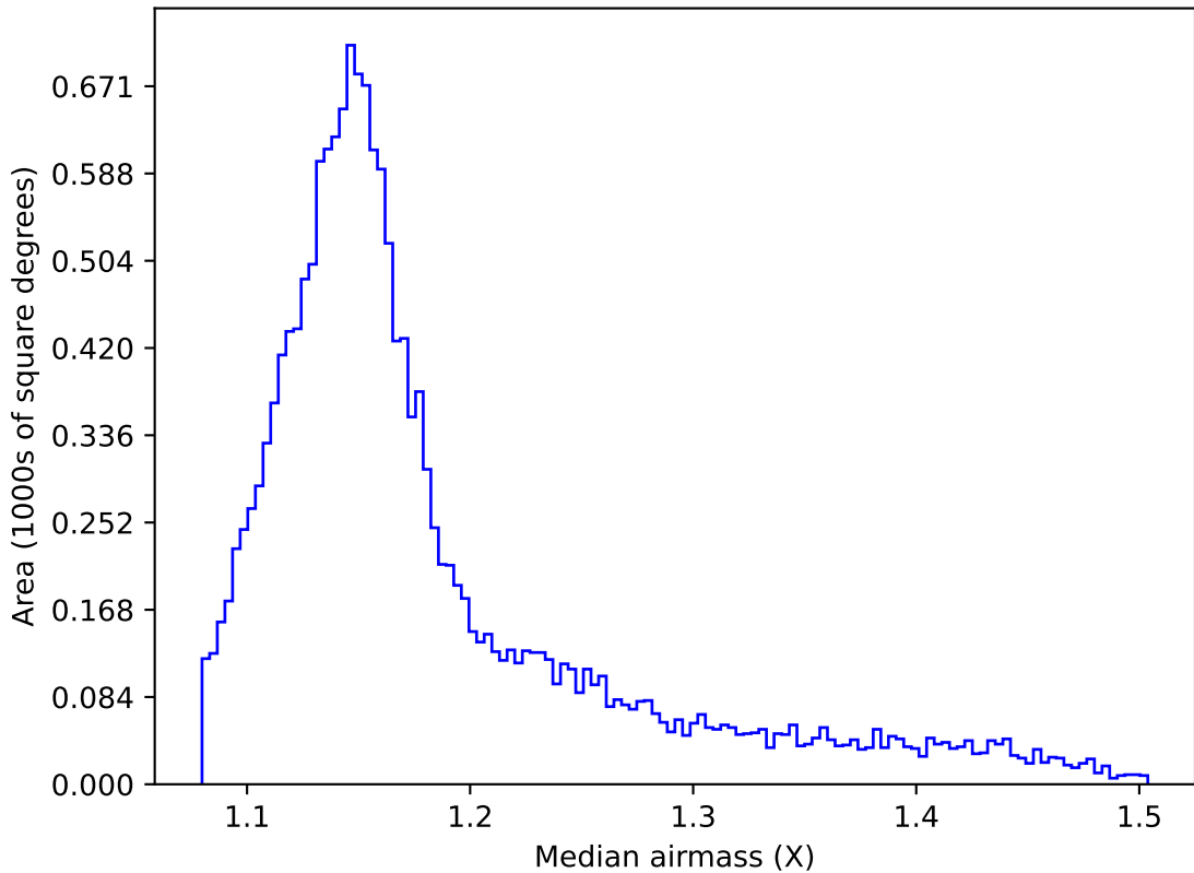
weather_cloudso31v3.4_10yrs WFD r band: Median airmass
