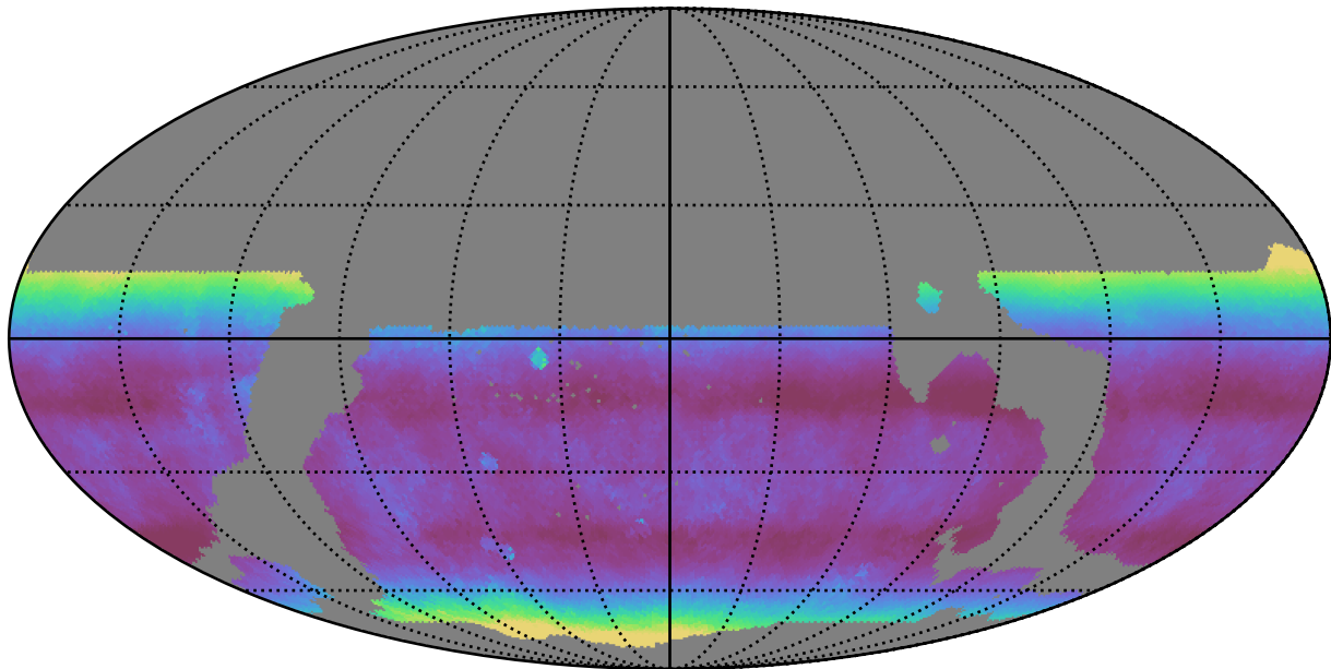
weather_cloudso31v3.4_10yrs WFD i band: Median airmass
