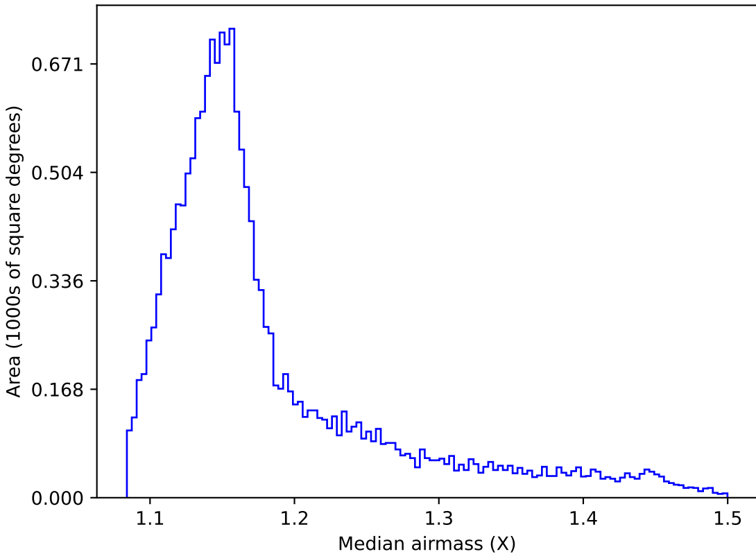
weather_cloudso31v3.4_10yrs WFD i band: Median airmass
