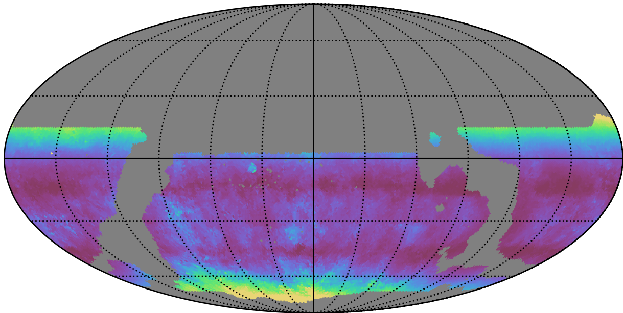
weather_cloudso31v3.4_10yrs WFD g band: Median airmass
