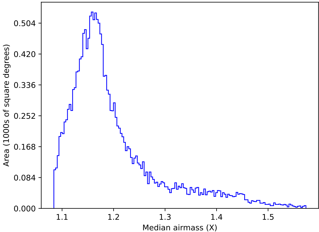
weather_cloudso31v3.4_10yrs WFD g band: Median airmass
