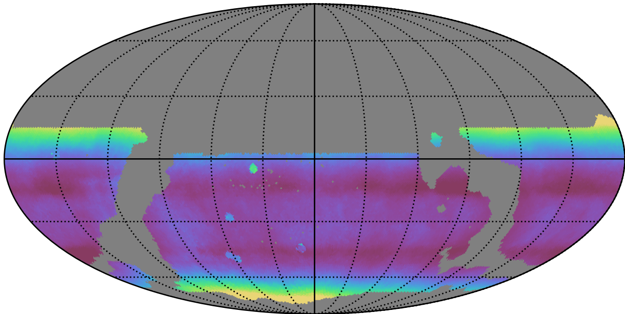
weather_cloudso31v3.4_10yrs WFD all bands: Median airmass
