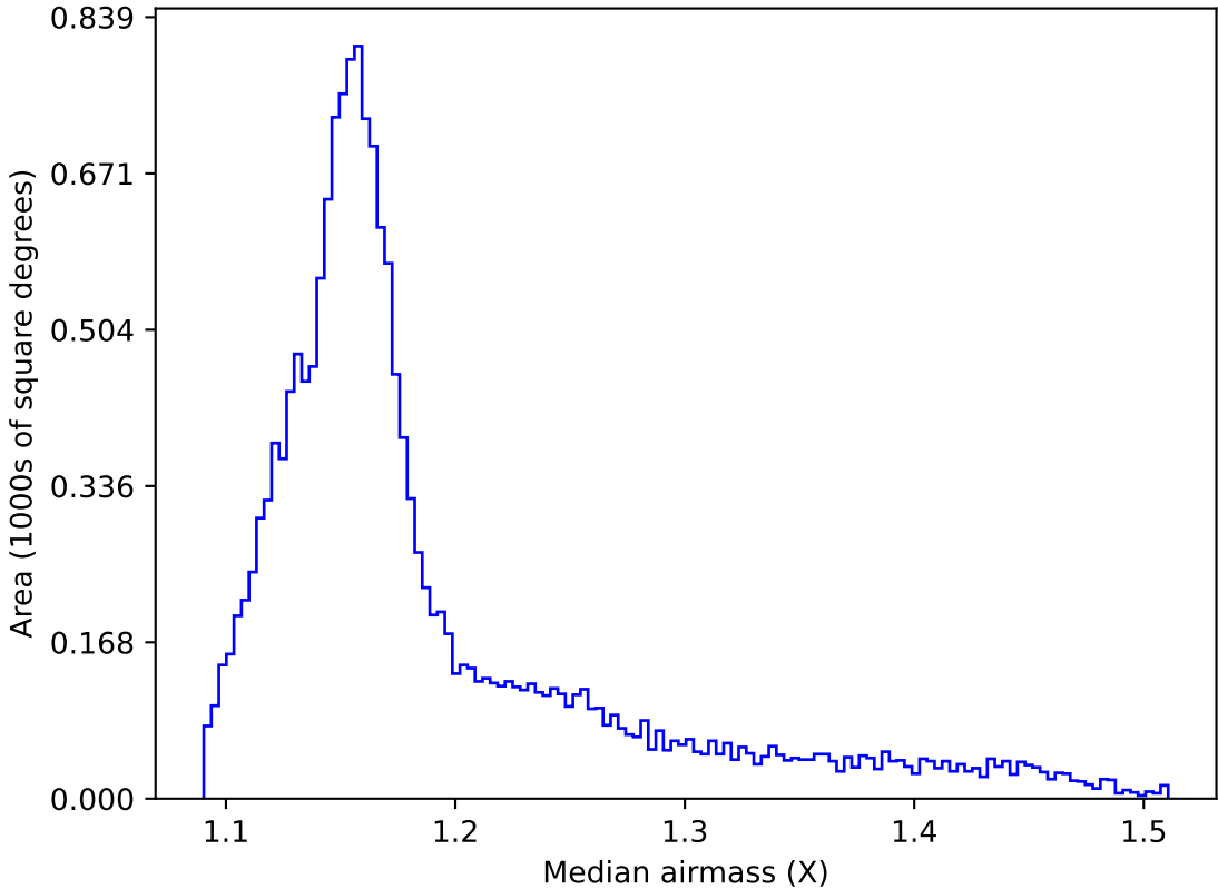
weather_cloudso31v3.4_10yrs WFD all bands: Median airmass
