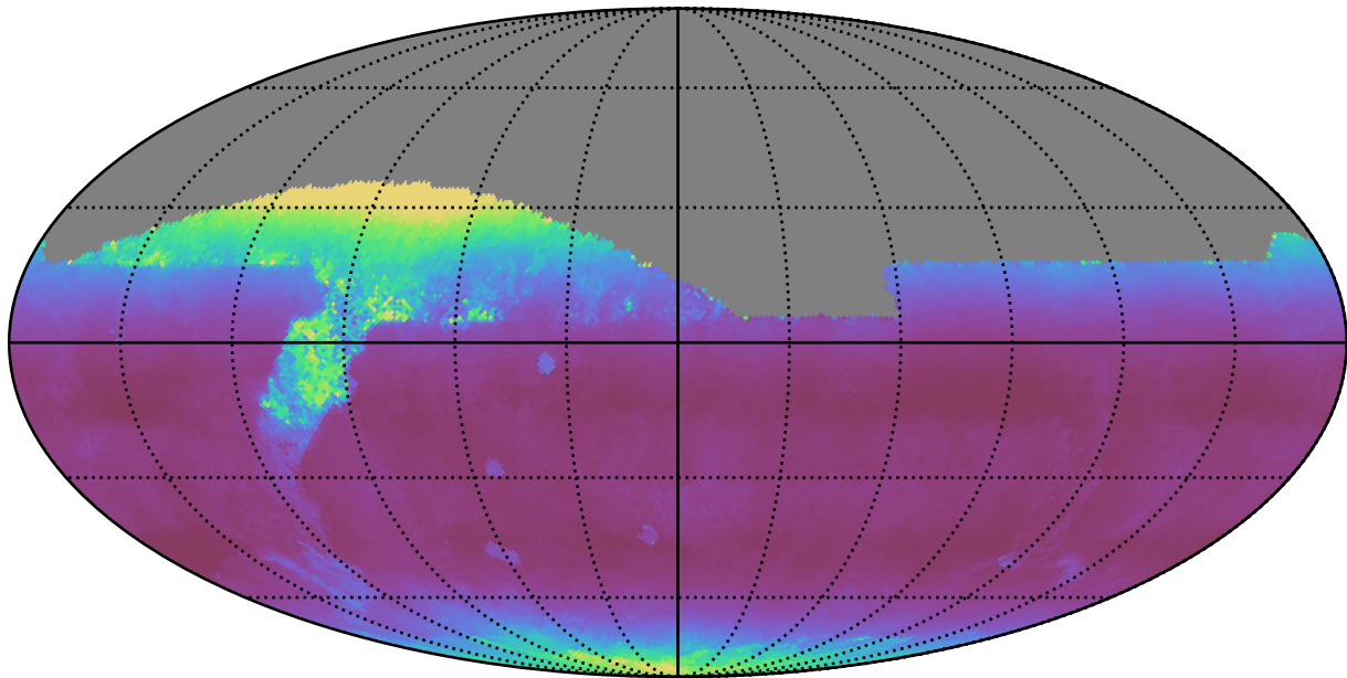
weather_cloudso31v3.4_10yrs All sky z band: Median airmass
