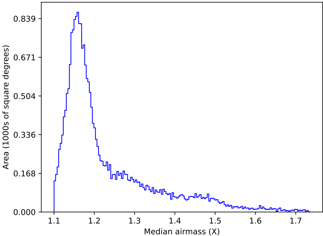
weather_cloudso31v3.4_10yrs All sky y band: Median airmass
