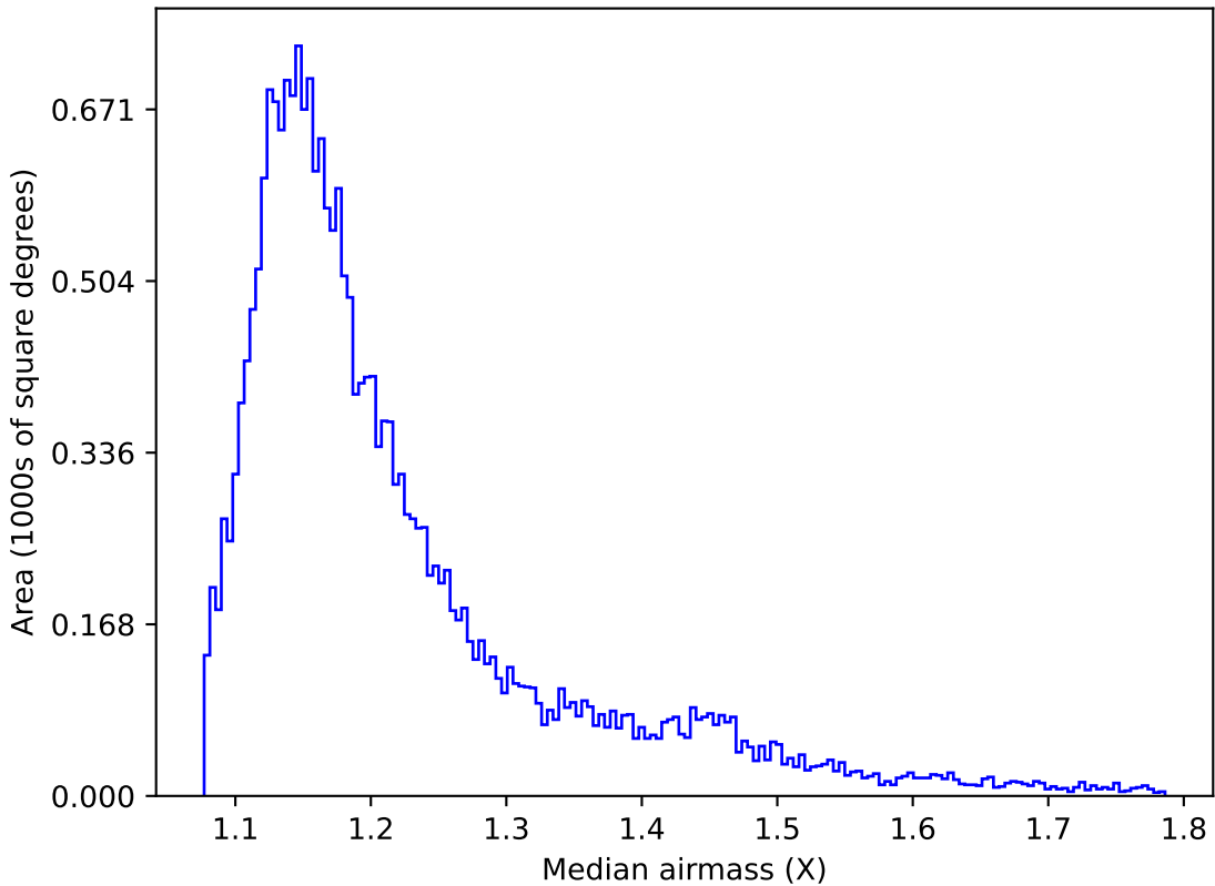
weather_cloudso31v3.4_10yrs All sky u band: Median airmass
