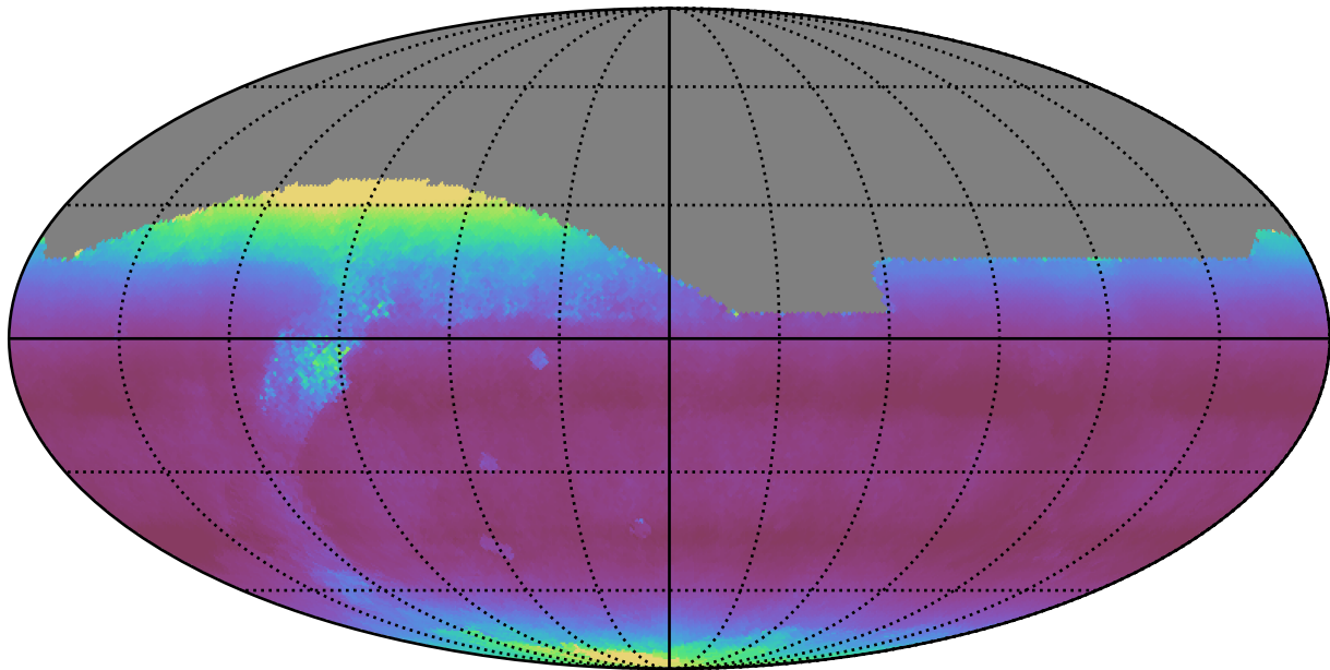
weather_cloudso31v3.4_10yrs All sky r band: Median airmass
