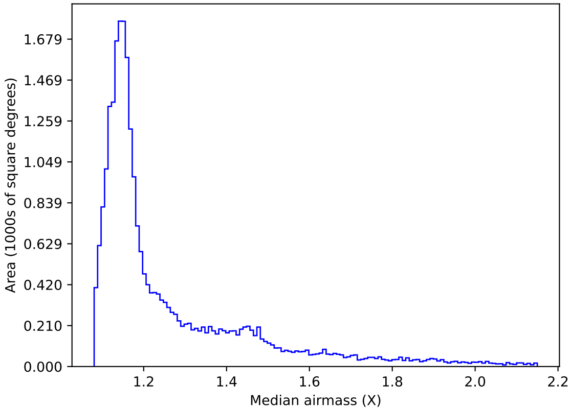
weather_cloudso31v3.4_10yrs All sky r band: Median airmass
