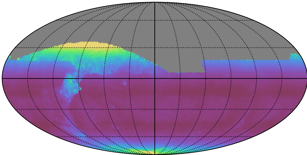
weather_cloudso31v3.4_10yrs All sky i band: Median airmass
