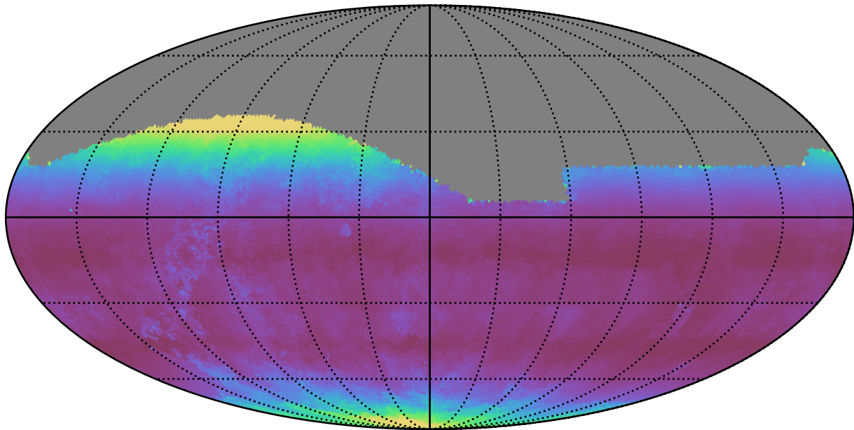
weather_cloudso31v3.4_10yrs All sky g band: Median airmass
