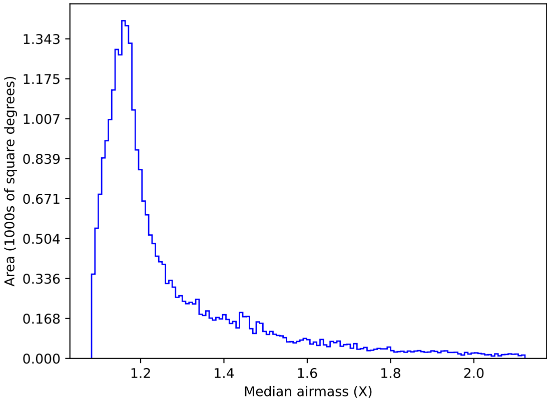
weather_cloudso31v3.4_10yrs All sky g band: Median airmass
