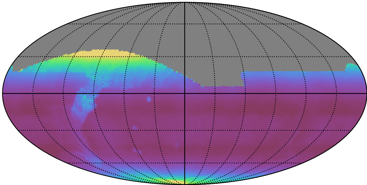
weather_cloudso31v3.4_10yrs All sky all bands: Median airmass
