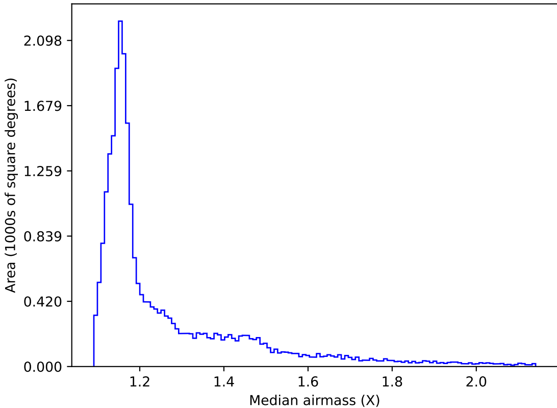
weather_cloudso31v3.4_10yrs All sky all bands: Median airmass
