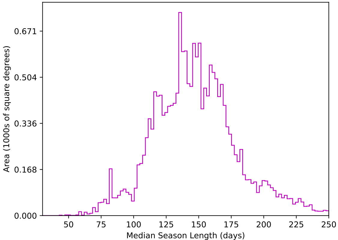
weather_cloudso31v3.4_10yrs WFD z band: Median Season Length
