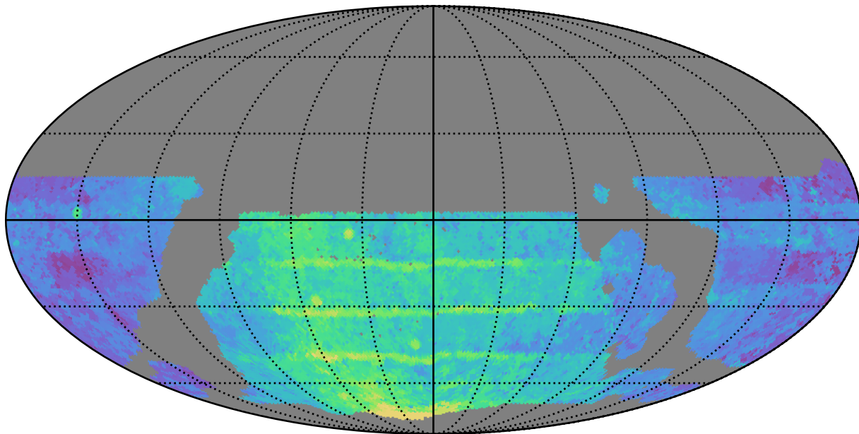
weather_cloudso31v3.4_10yrs WFD y band: Median Season Length
