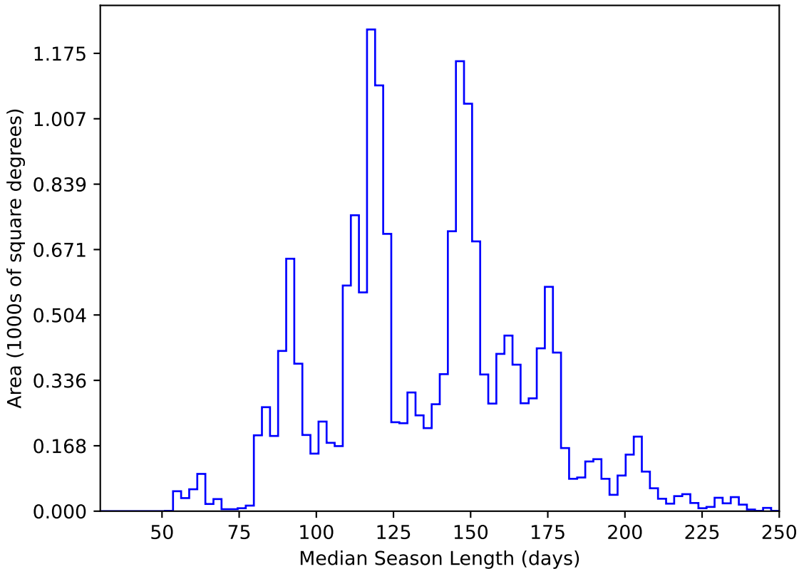
weather_cloudso31v3.4_10yrs WFD y band: Median Season Length
