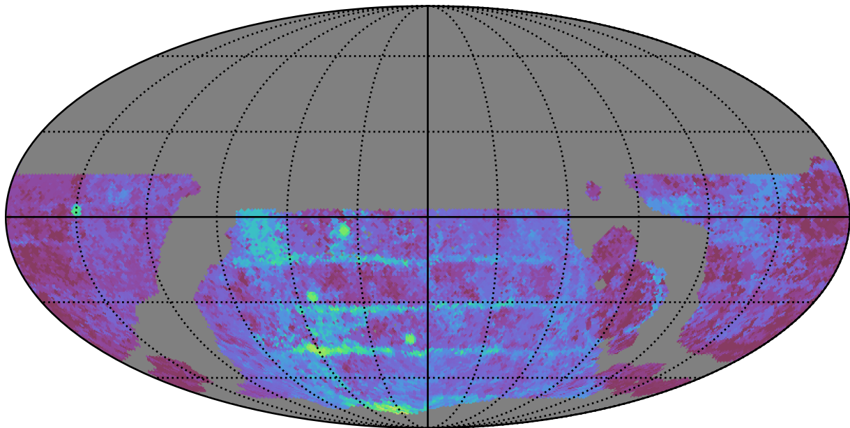
weather_cloudso31v3.4_10yrs WFD u band: Median Season Length
